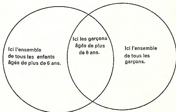
Fig. 7 INTERSECTION
